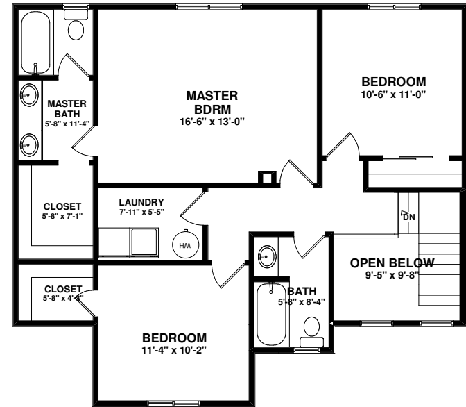
UPPER LEVEL FLOOR PLAN 813 sq ft
