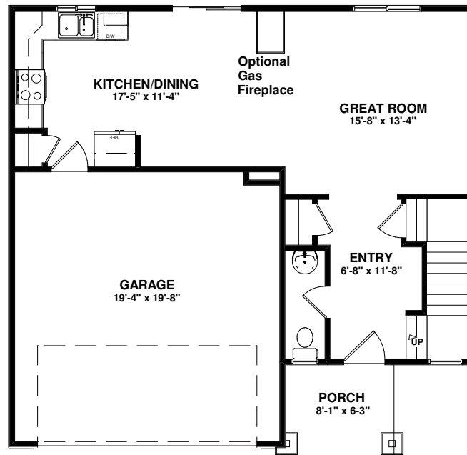
MAIN LEVEL FLOOR PLAN 601 sq ft
